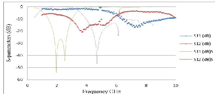
Figure 10. Measured and Simulated Response of Fabricated Prototype II Circuit.
