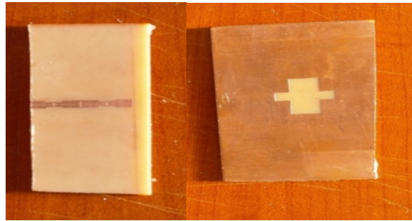
Figure 13. Photograph of Fabricated Prototype III Circuit (grooves in all sections).
